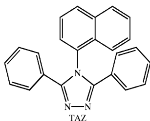
TAZ
