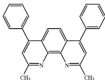
BC
