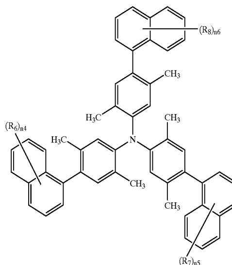
formula (II)
